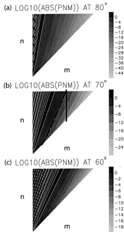
FIG. 1. Logarithm scale with base 10 of the absolute amplitude of the associated Legendre function, for T62 near the latitudes of (a) 80°, (b) 70°, and (c) 60°N. The black solid line in (b) indicates the trapezoidal spectral summation, and the dashed line indicates the scalenelike spectral summation. The white contours are zero values that indicate the unit of magnitude of the associated Legendre coefficient.
